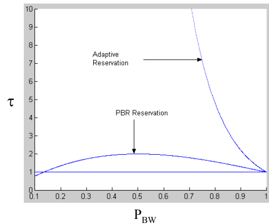
Fig6. Comparison parameter \tau plotted as function of P_{BW}
