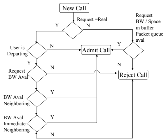
Fig 5. Flow chart of call admission control
