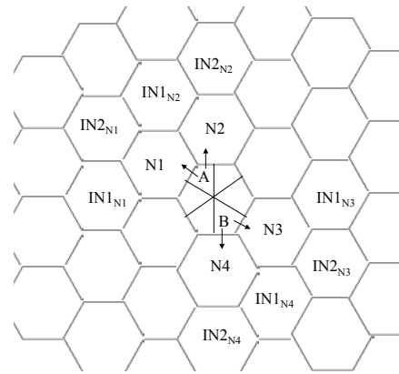
Fig4. Nearest neighbor and immediate neighbor for bandwidth reservation / possible borrowing.
